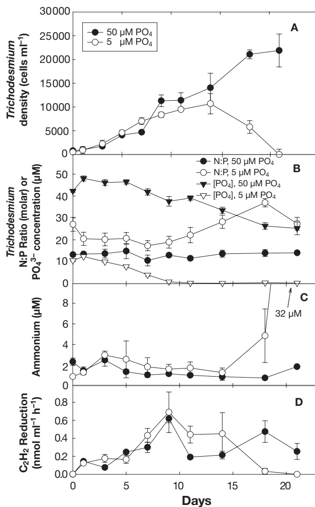
Fig. 3. Trichodesmium IMS 101 growth curve 2. (A) Cell counts, (B) N:P ratio and PO 4 3- concentrations, (C) ammonium concentrations and (D) C 2 H 2 reduction rates. Error bars are ±SE
