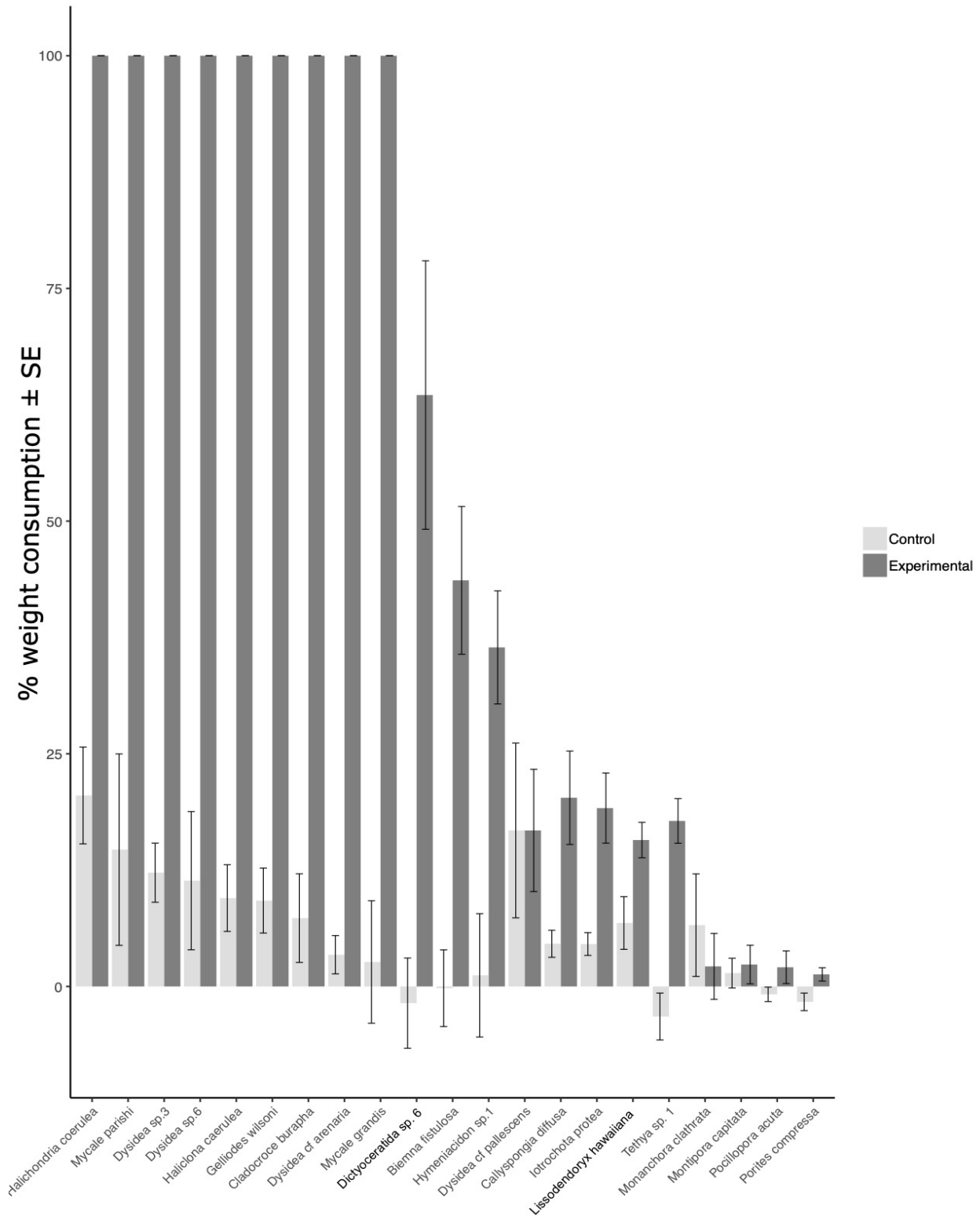
Figure S1 Mean and standard error of % weight consumption of control and experimental prey species after 144 h. Experimental prey species were exposed to cowries while control prey species were isolated from predators in an adjacent wet table.
