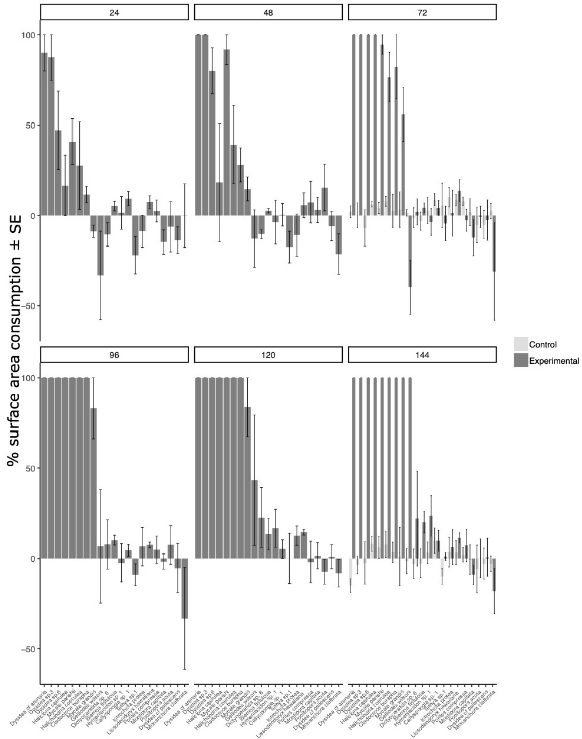
Figure S2 Mean and standard error of % surface area consumption (%) of sponge species that were completely consumed, at 24-h intervals over 144-h period. Experimental prey species were exposed to cowries while control prey species were isolated from predators in an adjacent wet table.
