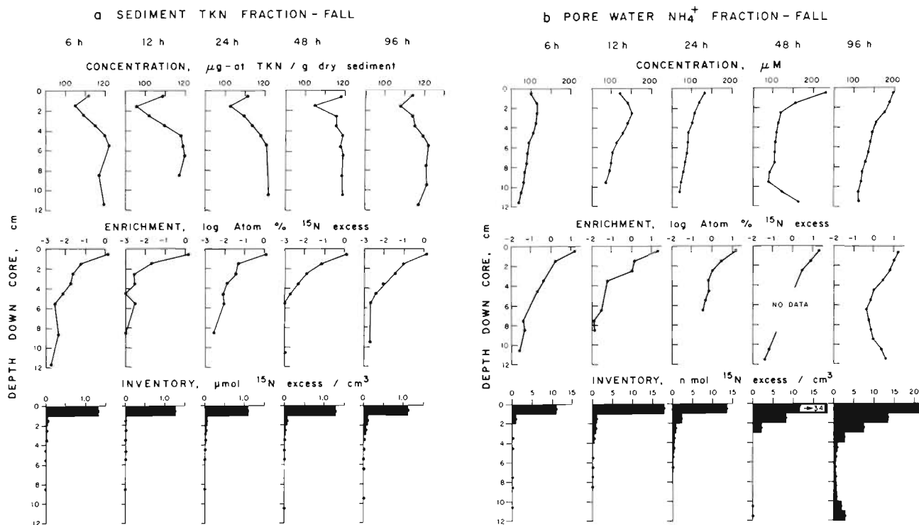
Fig. 3. Fall experiment: profiles of nitrogen concentrations, ^{15}\text{N} enrichments and ^{15}\text{N} inventories in sediment TKN (a), and porewater \text{NH}_4^+ (b), at various times after cores were treated with ^{15}\text{N} -labelled PON
