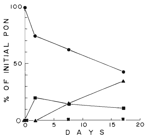
Fig. 4. Dynamics of the aerobic decomposition of ^{15}\text{N} -labelled Skeletonema costatum cells in glass-fiber-filtered Narragansett Bay water, 8^\circ\text{C} . Initial amount of PON (0.73 mg-at N), identical to that added to sediment cores, was suspended in 11 of bay water. Circles: PON; squares: DON; triangles: \text{NH}_4^+ ; crosses: \text{NO}_2^- + \text{NO}_3^-
