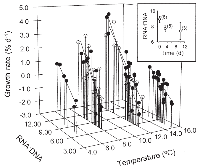
Fig. 4. Gadus morhua and Melanogrammus aeglefinus . RNA:DNA and growth rate data collected at 5, 8, 12, and 15°C for cod ( n = 56 , ●) and at 8 and 12°C for haddock ( n = 32 , ○). Each datum equals the mean RNA:DNA and growth rate for the 3 fish in each tank. Linear regression equations and statistics are provided in Table 5. Insert: mean \pm SE RNA:DNA versus time since last feeding (d) at 8.0°C for 6.1 to 8.2 cm SL haddock. No. of fish sampled at each time is indicated in parentheses
