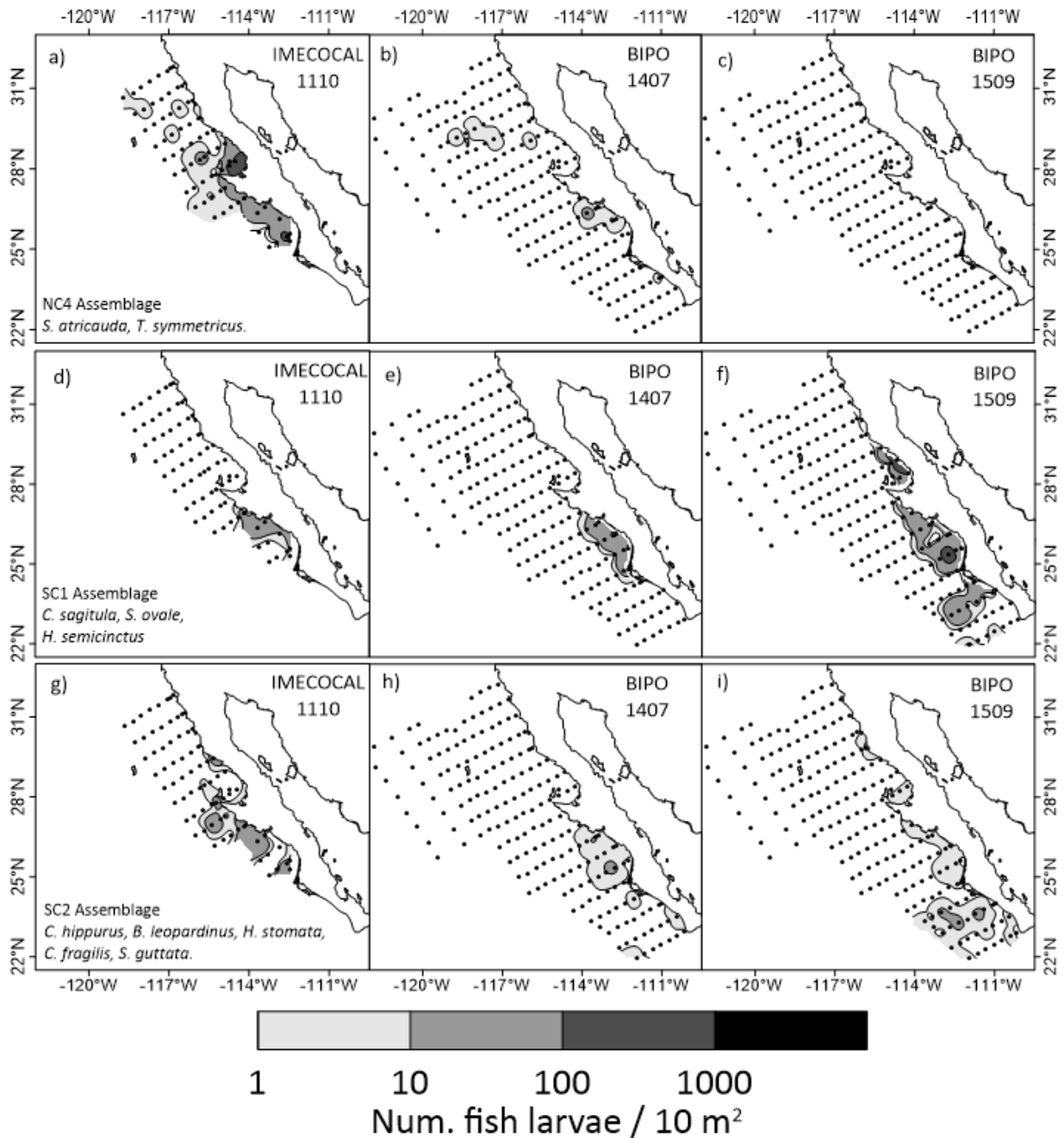
Figure S2. Distribution of the fish larvae assemblages NC4, SC1, and SC2 during the summer-fall seasons of 2011 and 2014-2015.
