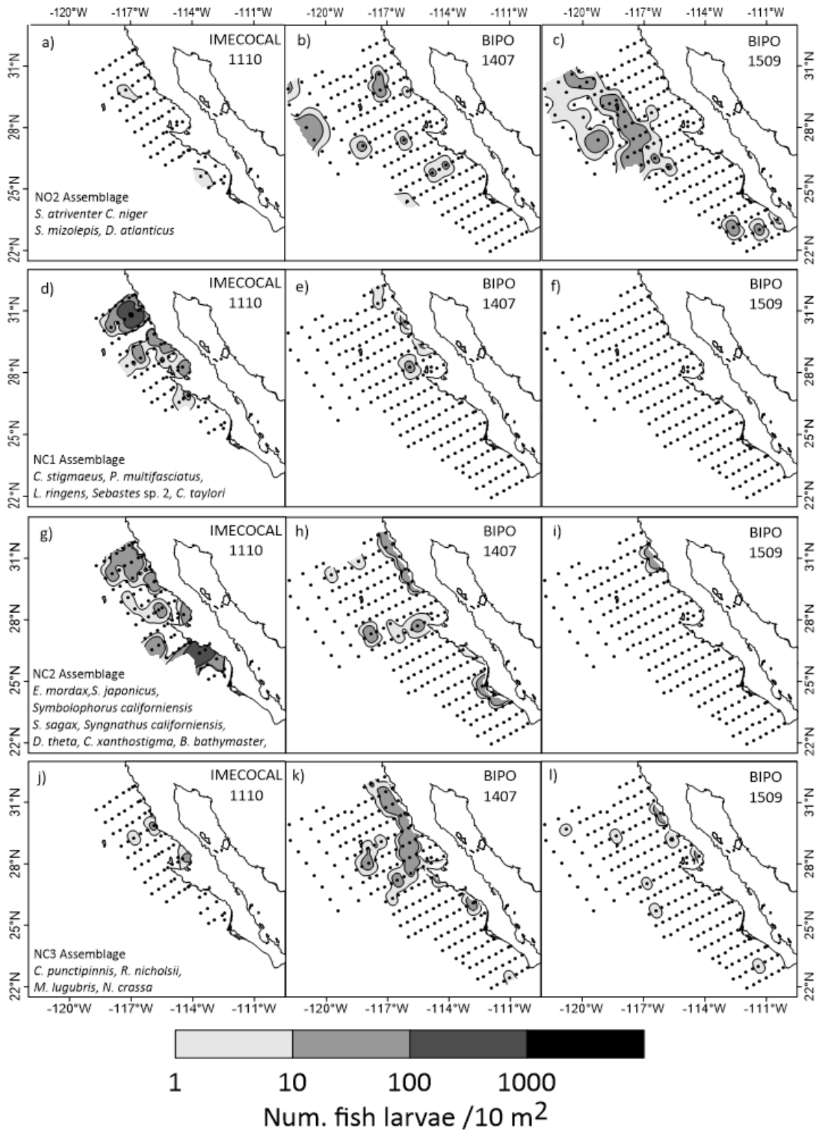
Figure S1. Distribution of the fish larvae assemblages NO2, NC1, NC2, and NC3 during the summer-fall seasons of 2011 and 2014-2015.
