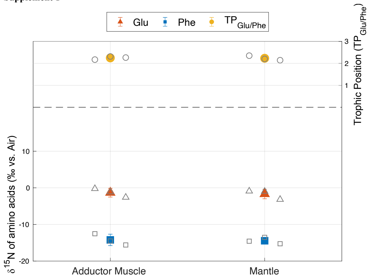
Fig. S1. \delta^{15}\text{N} of glutamic acid ( \delta^{15}\text{N}_{\text{Glu}} ), phenylalanine ( \delta^{15}\text{N}_{\text{Phe}} ), and trophic position ( \text{TP}_{\text{Glu/Phe}} ) for adductor muscle and mantle of Phreagena okutanii .
