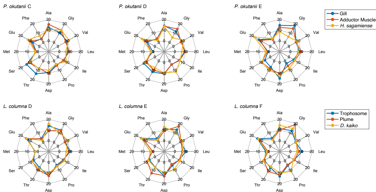
Fig. S2. Radar chart for relative concentration data (%) of 12 amino acids in the Phreagena-Hyphalion association and the Lamellibrachia-Dirivultus association.
