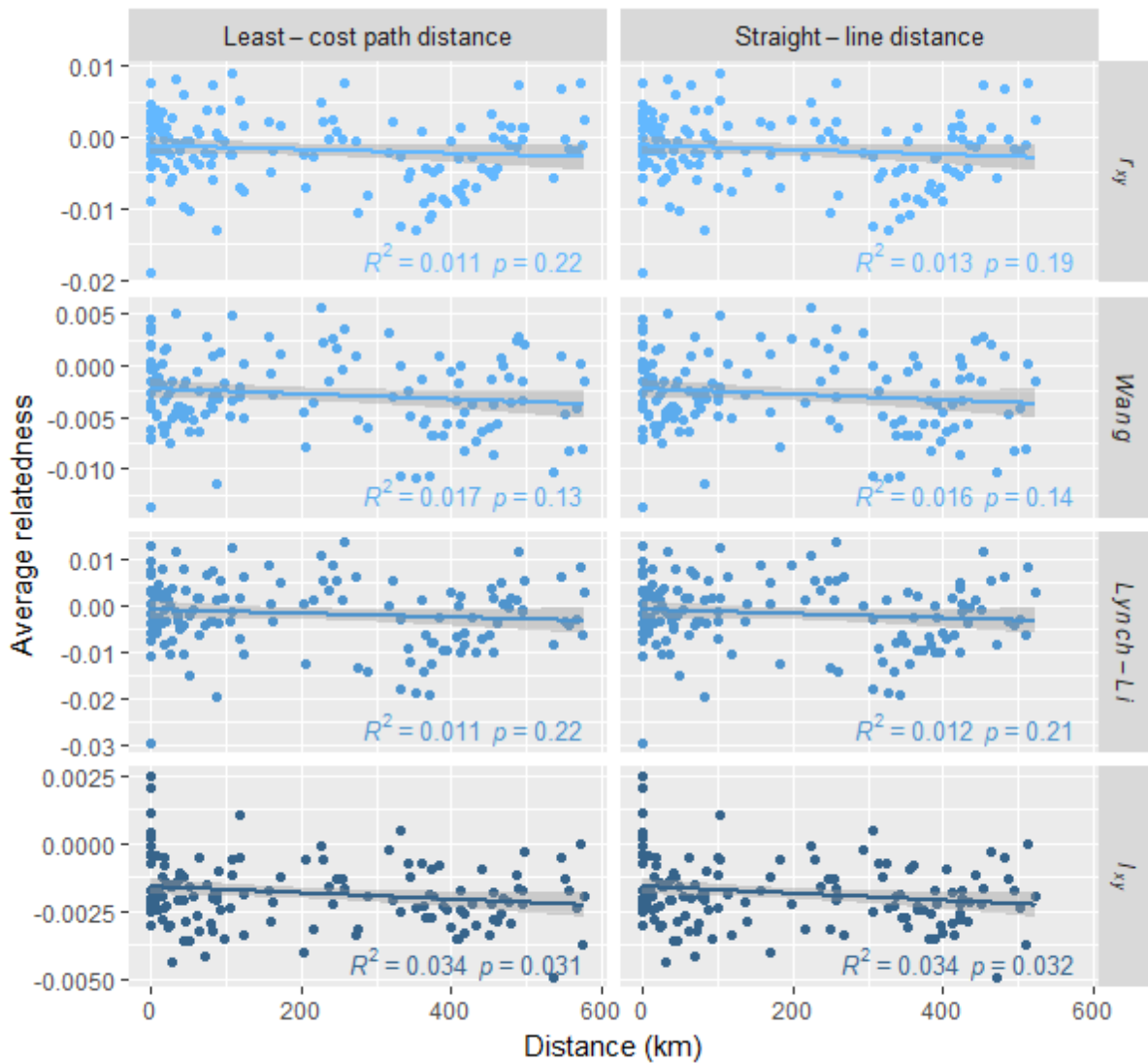
Fig. S6: Average relatedness for four common estimators according to geographic distance. R^2 and p -values correspond to linear regressions.
