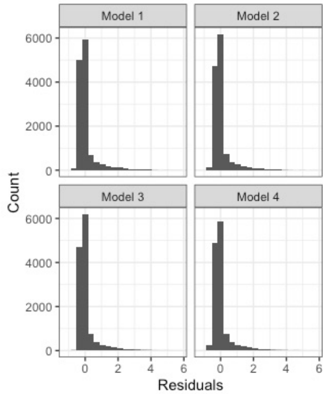
Figure S3: Distributions of model residuals for the four generalized additive models ran on the second length bin (20-30cm). These residuals incorporate fixed effects only and treat random effects as error.
