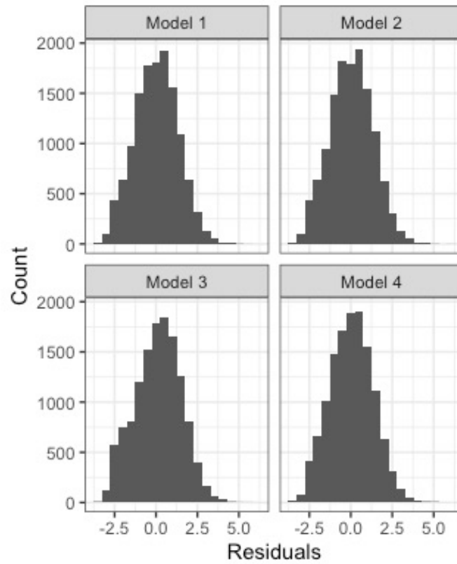
Figure S6: Distributions of model residuals for the four generalized additive models ran on the fifth length bin (>50cm). These residuals incorporate fixed effects only and treat random effects as error.
