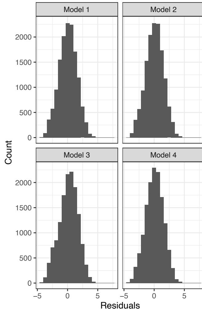
Figure S1: Distributions of model residuals for the four main (all ages) generalized additive models. These residuals incorporate fixed effects only and treat random effects as error.
