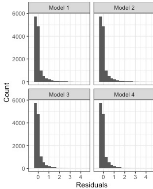
Figure S2: Distributions of model residuals for the four generalized additive models ran on the first length bin (0-20cm). These residuals incorporate fixed effects only and treat random effects as error.
