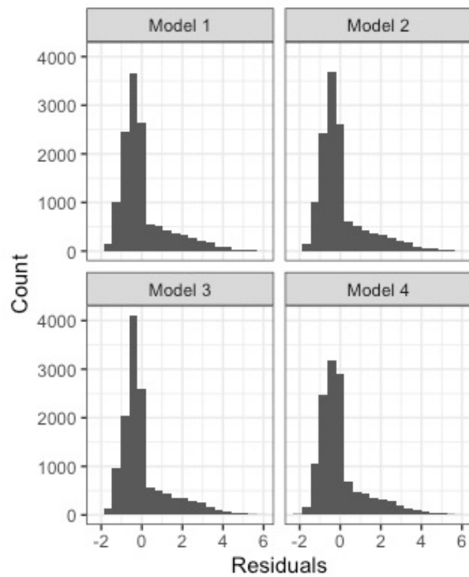
Figure S4: Distributions of model residuals for the four generalized additive models ran on the third length bin (30-40cm). These residuals incorporate fixed effects only and treat random effects as error.
