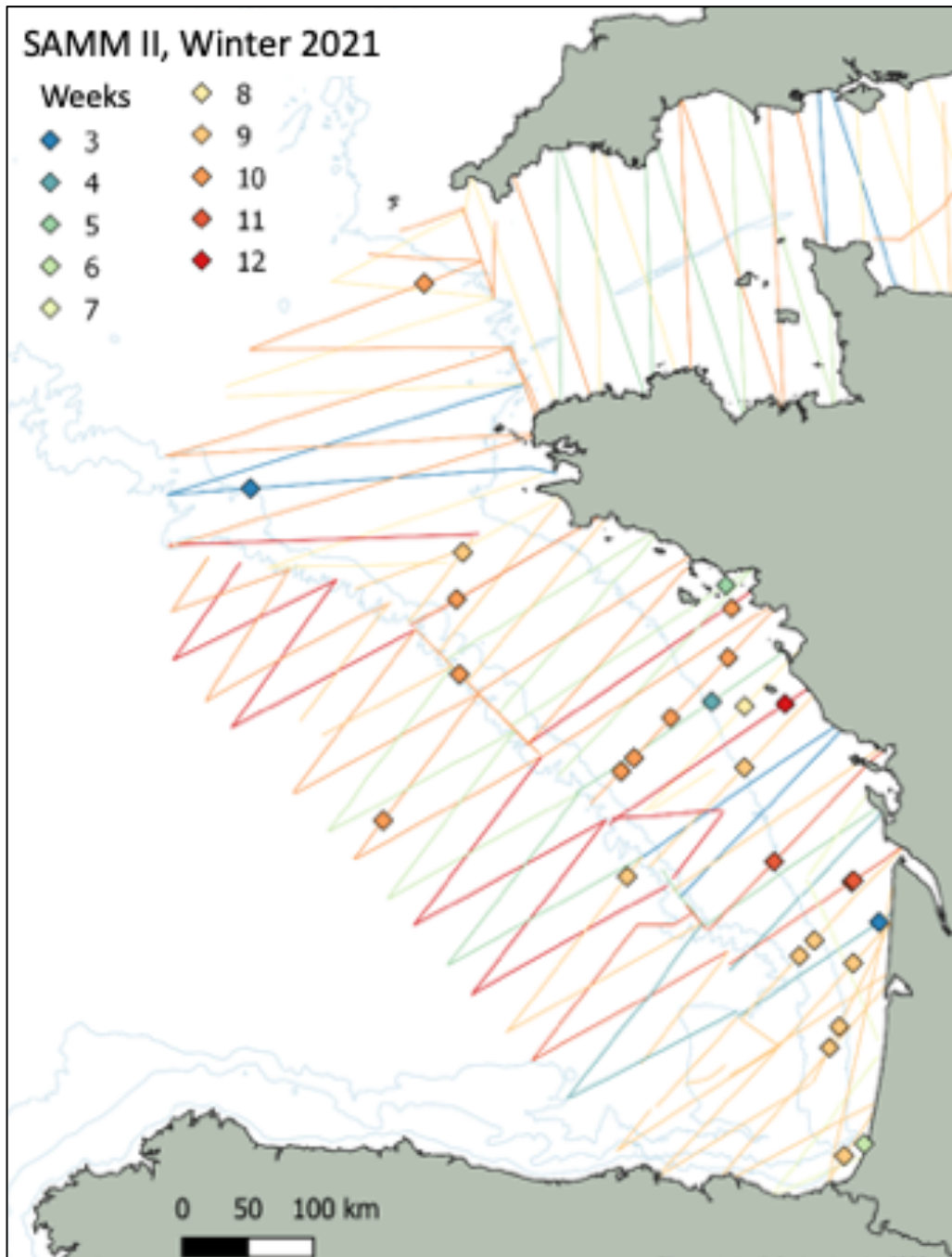
Fig. S1. Locations of small delphinid drifting carcasses recorded during the SAMM-II survey by week of the winter 2021. Carcass observations and the effort associated with the week's resolution are shown in the same color.
